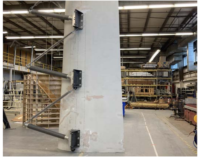
BladePole mock-up in laboratory
